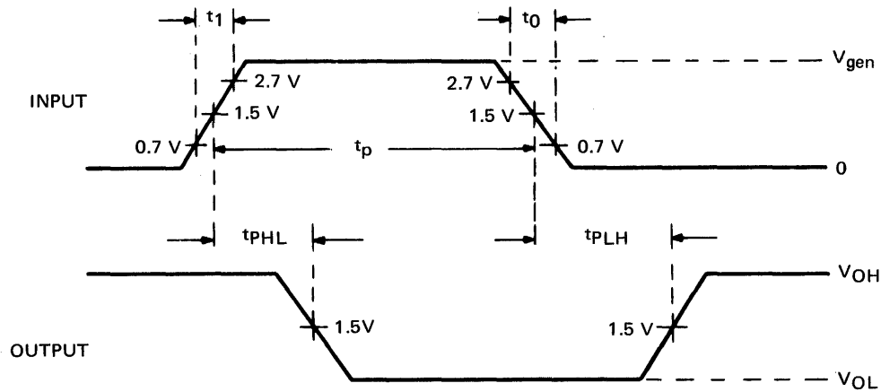
VOLTAGE WAVEFORMS
