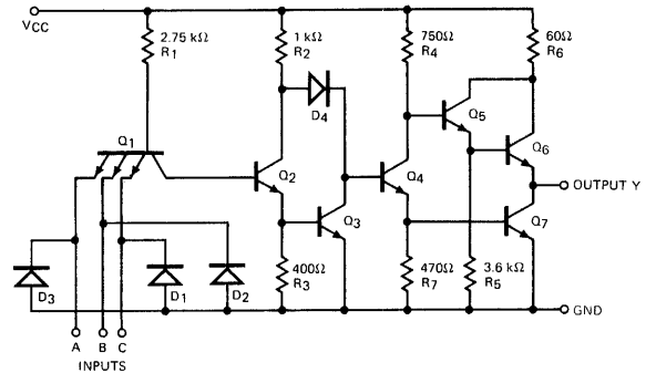
SCHEMATIC DIAGRAM (EACH GATE)
