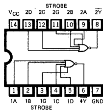
DIP (TOP VIEW)
