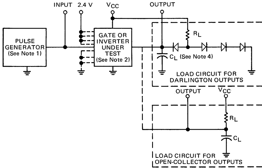
TEST CIRCUIT
