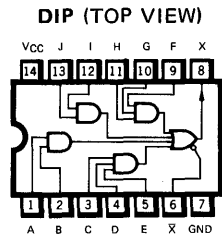
LOGIC AND CONNECTION DIAGRAM
