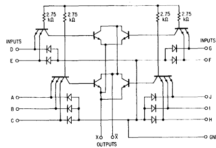
SCHEMATIC DIAGRAM
