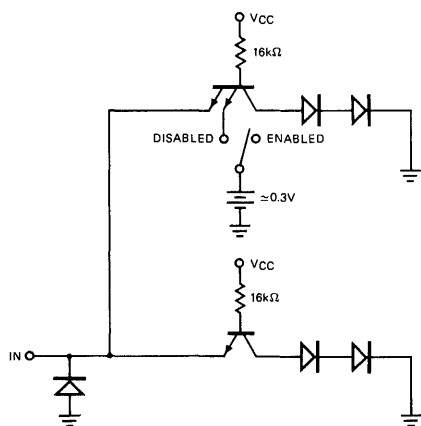
INPUTS EQUIVALENT CIRCUIT
