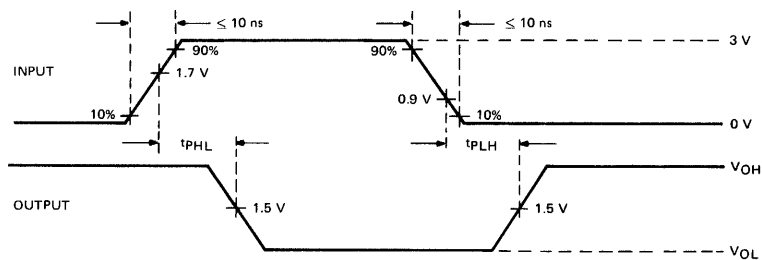
VOLTAGE WAVEFORMS
