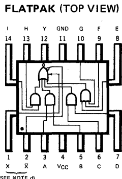
LOGIC AND CONNECTION DIAGRAM
