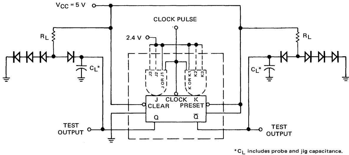
TEST CIRCUIT
