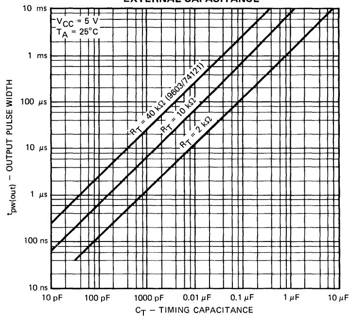
Fig. 8 OUTPUT PULSE WIDTH VERSUS EXTERNAL CAPACITANCE
