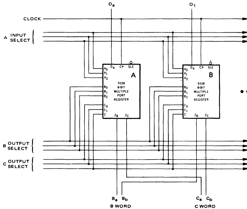
Fig. 9 PARALLEL EXPANSION
