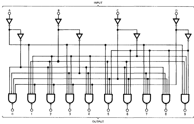
LOGIC DIAGRAM 9354/5444, 7444 EXCESS 3 GRAY-TO-DECIMAL
