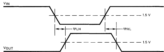
SWITCHING WAVEFORM
