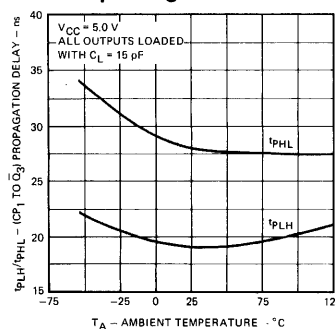
TYPICAL PROPAGATION DELAY VERSUS TEMPERATURE CP 1 TO Q 3 MODULO 8
