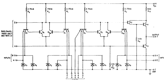
SCHEMATIC DIAGRAM
