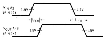
t_{PLH}/t_{PHL} - A_2 \text{ to } A = B
