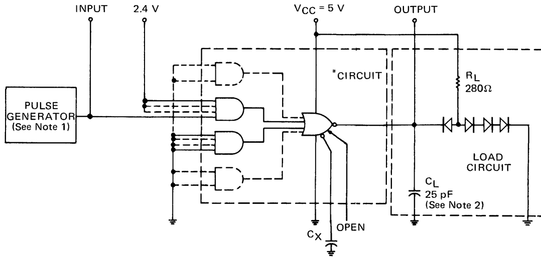
TEST CIRCUIT
