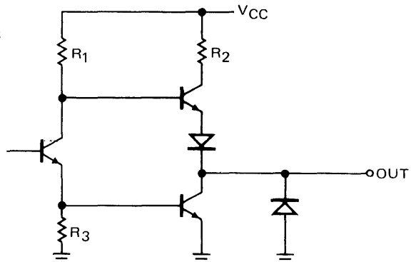
TYPICAL RESISTORS
