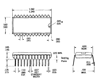
24 Lead Plastic MSI Dual In-line
