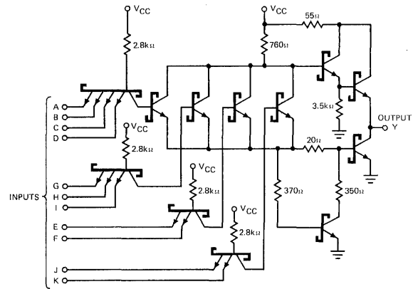
SCHEMATIC DIAGRAM
