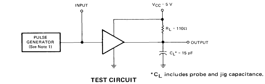
Fig. J PROPAGATION DELAY TIMES
