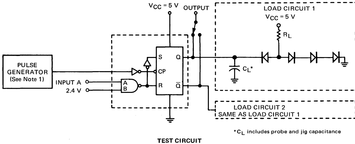
TEST CIRCUIT
