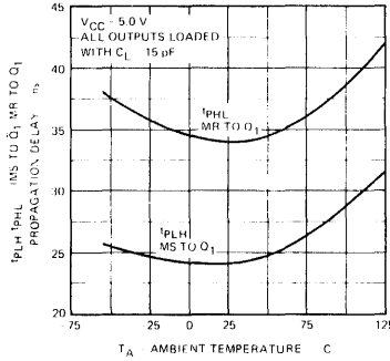
TYPICAL PROPAGATION DELAY VERSUS TEMPERATURE t PLH MS TO Q 1 t PHL MR TO Q 1 MODULO 8
