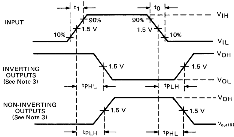
VOLTAGE WAVEFORMS
