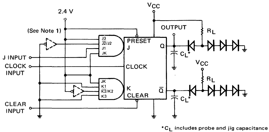
TEST CIRCUIT
