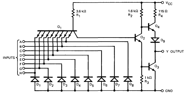
SCHEMATIC DIAGRAM
