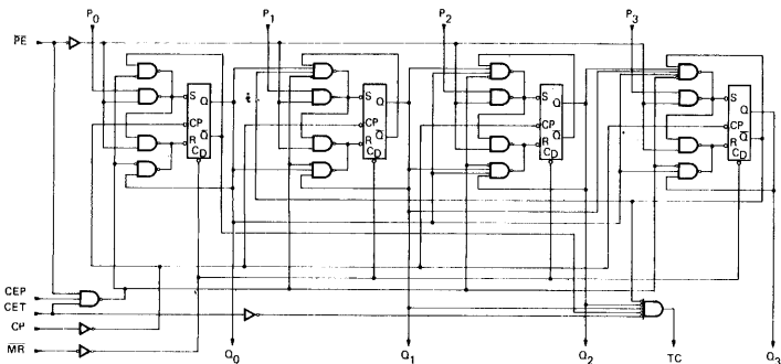
LOGIC DIAGRAM 9310
