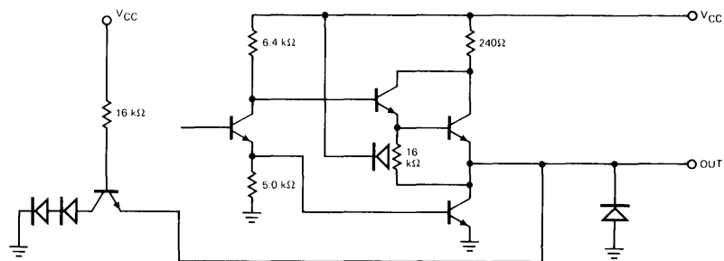
OUTPUTS EQUIVALENT CIRCUIT
