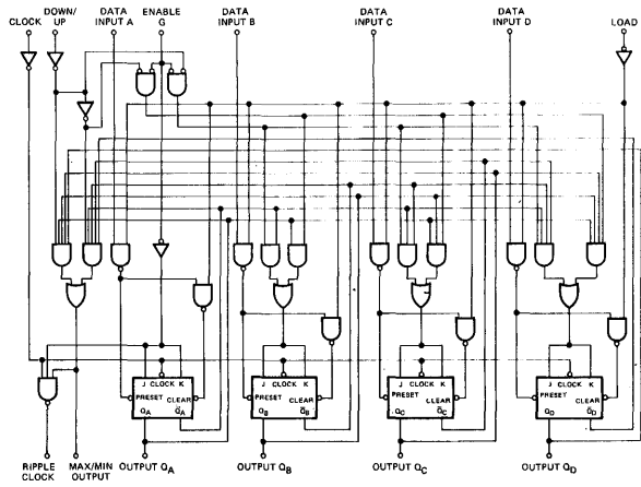
BINARY COUNTER 93191/54191, 74191
