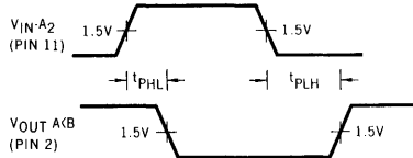
t_{PLH}/t_{PHL} - A_2 \text{ to } A < B
