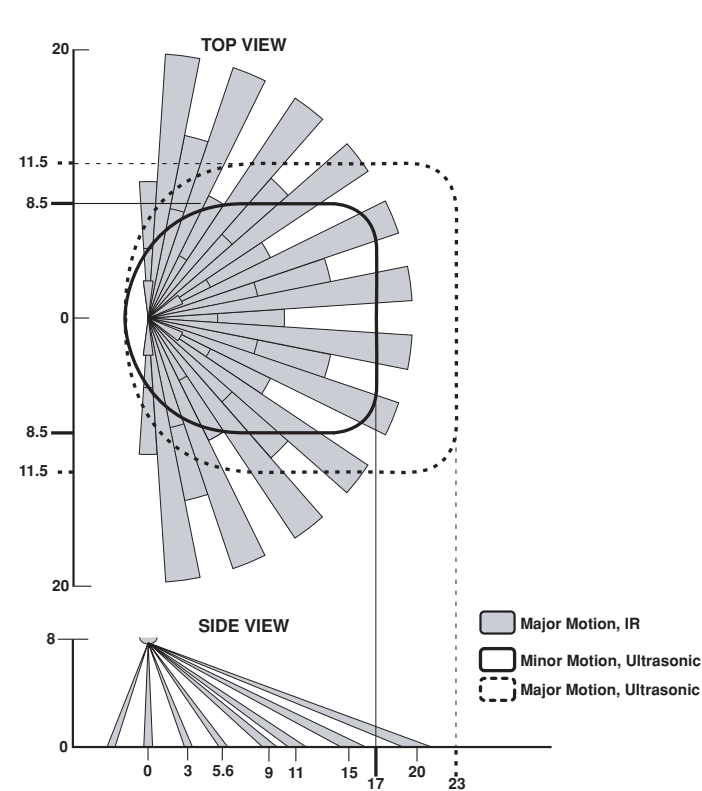
Figure 2 (Cat. No. OSC05) Field-of-View Ranges
