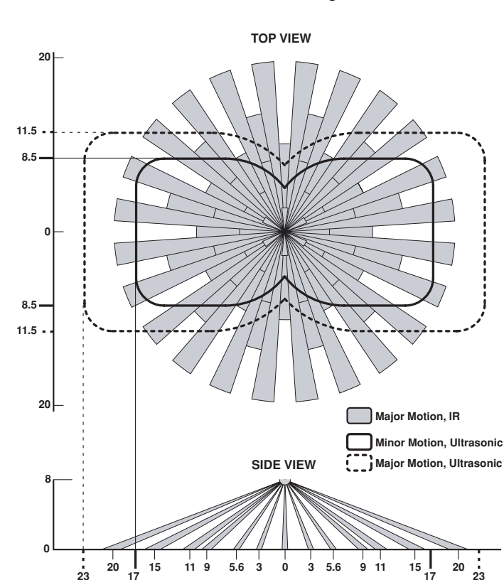
Figure 3 (Cat. No. OSC10) Field-of-View Ranges
