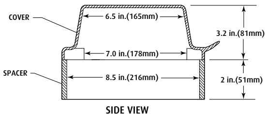
MODELS WITHOUT HORN (STI-1200 AND STI-3150 Series)
